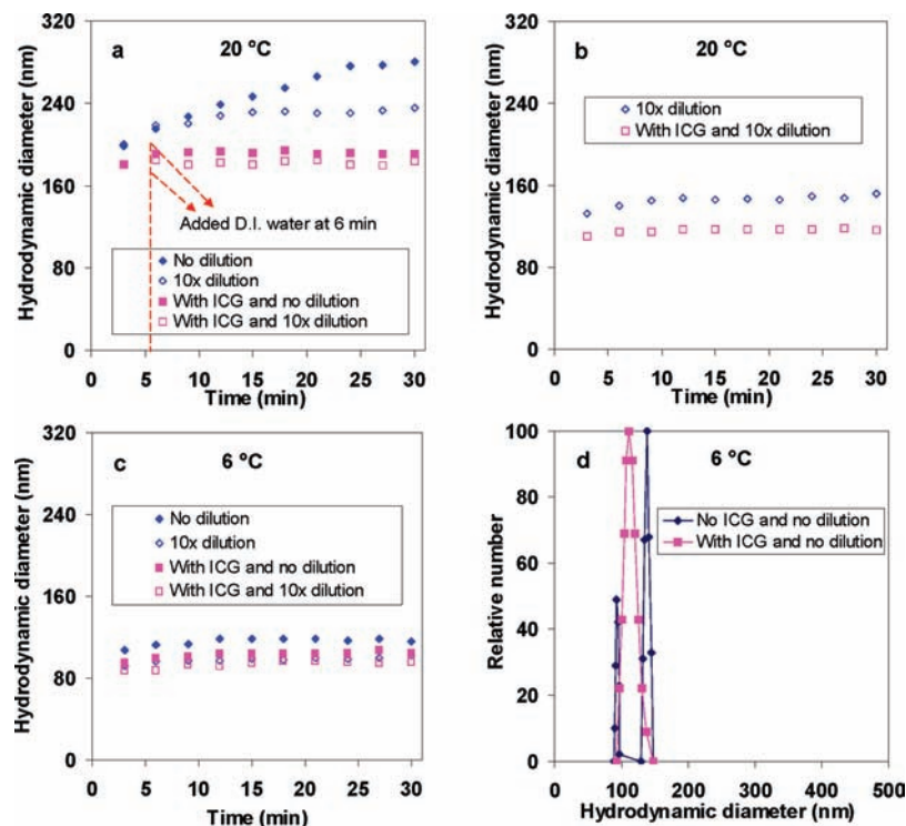
Figure 2. DLS study on PAH/phosphate aggregate and PAH/phosphate/ICG aggregate growth behavior ( R = 3 ) under the effects of 10 \times dilution and synthesis temperatures: (a) delayed dilution after aggregate formation at 20 °C; (b) immediate dilution after aggregate formation at 20 °C; (c) aggregate formation at 6 °C and the effects of dilution and ICG inclusion; and (d) size distributions at 6 °C and 30 min.
