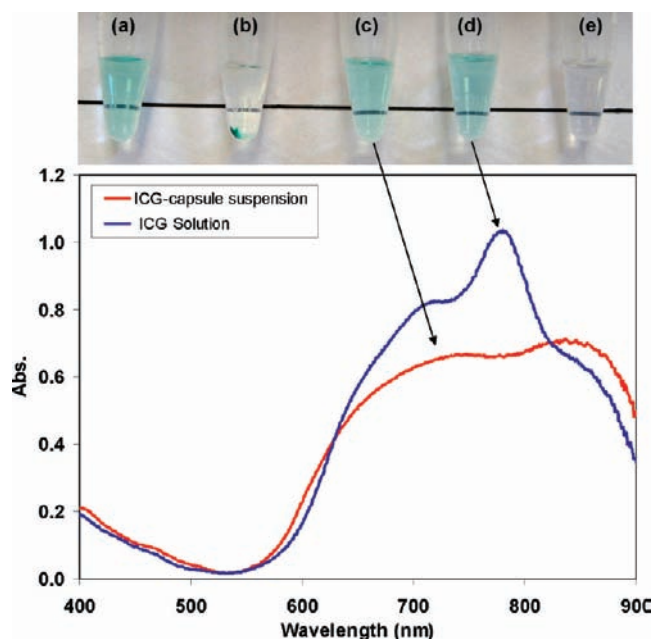
Figure 4. Absorbance spectra of nonencapsulated ICG in PBS solution (blue line) and ICG-containing anti-EGFR coated nanocapsule suspension (red line). The ICG concentration was adjusted to 0.03 mg/mL for these formulations (lower than the concentration used in the cell photothermal study). The photographs correspond to anti-EGFR-coated ICG-nanocapsules that (a) are stably suspended in PBS solution, (b) have settled out of suspension, and (c) redispersed back into suspension after sonication for 10 s; (d) nonencapsulated ICG in PBS solution; and (e) a suspension of PAH/HPO 4 2- aggregates.
