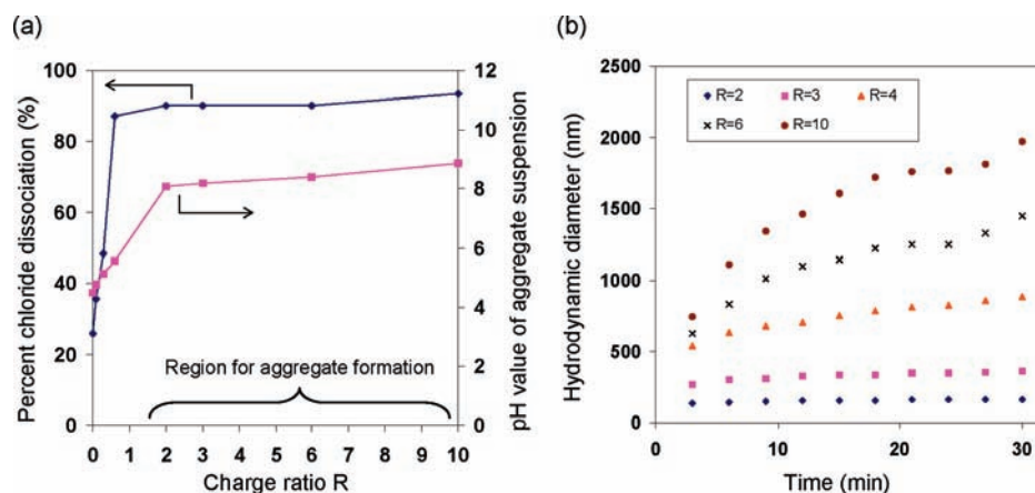
Figure 1. (a) Dissociated chloride percentages and corresponding pH values and (b) hydrodynamic diameters measured for PAH/phosphate aggregate suspensions as functions of R ratio. Aggregate formation conditions: temperature = 20 °C, PAH precursor solution concentration of 2 mg/mL, 1:6 volume ratio between PAH and \text{Na}_2\text{HPO}_4^{2-} precursor solutions.
