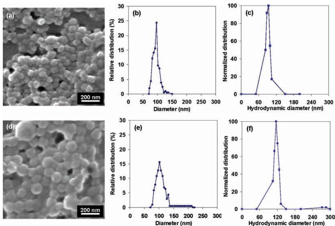
Figure 3. (a–c) SEM analysis of uncoated and (d–f) anti-EGFR-coated ICG-containing PAH/phosphate nanocapsules in dried stated: (a,d) SEM images and (b,e) particle size histograms, and (c,f) hydrodynamic diameter distributions of nanocapsules in water.
